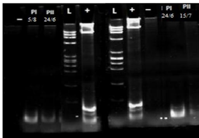
Figure 4. PCR results for the detection of toxic Microcystis in the Caspian Sea using primers specific to the Microcystis sp. mcyB gene. (+) Positive control, (-) Negative control, (L) Ladder.
